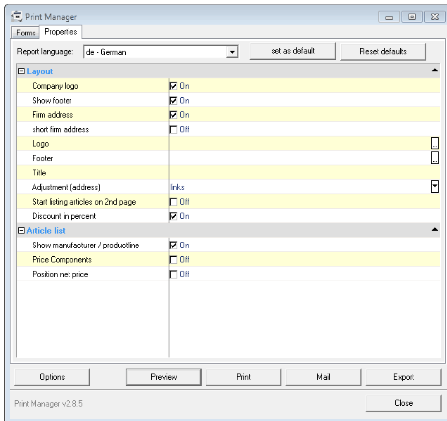
Properties window
