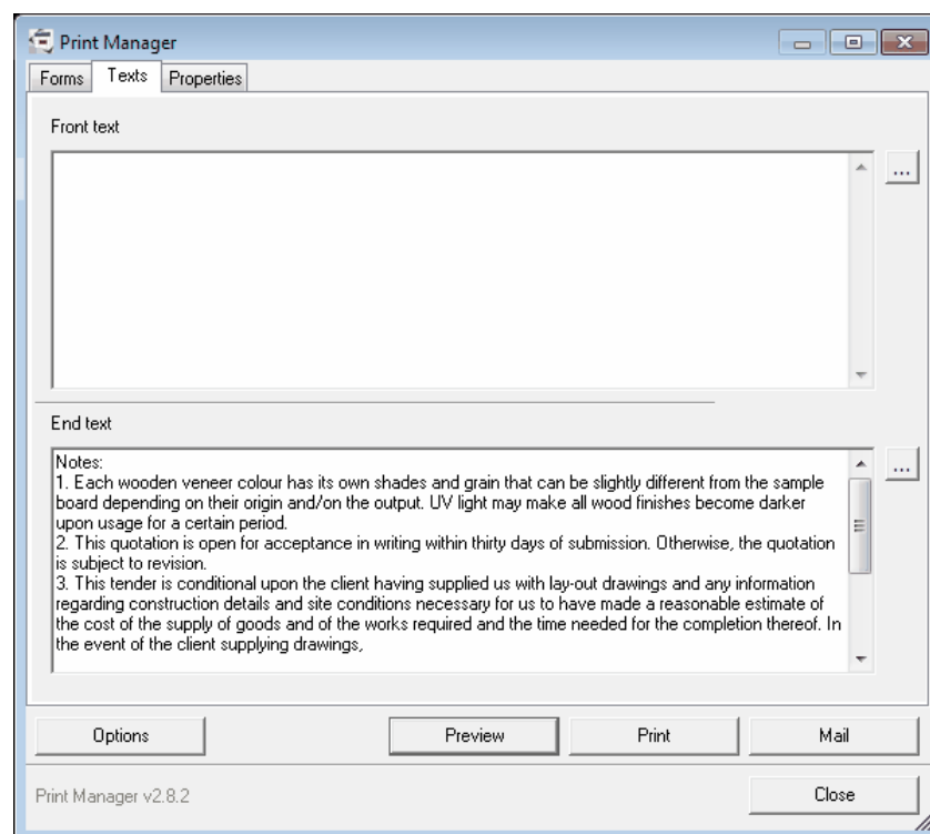
Texts window
