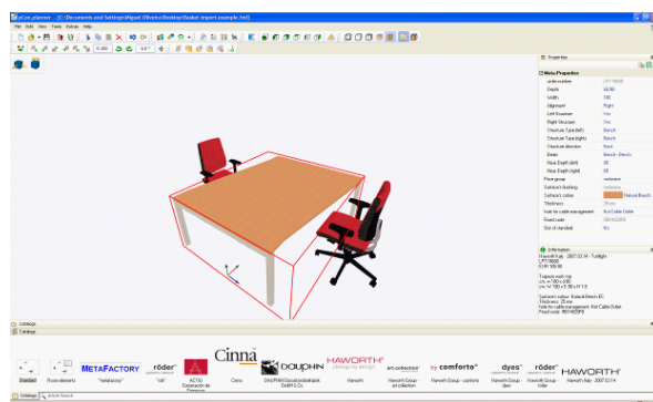
pCon.planner project
