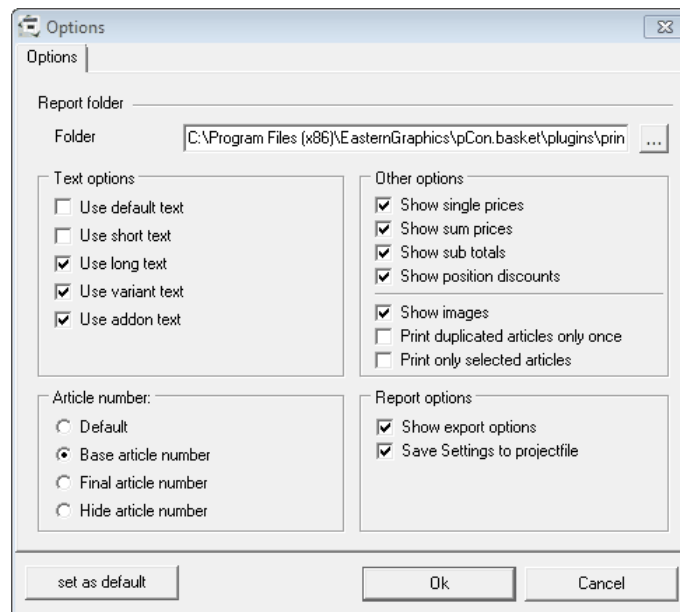
ReportManager Options
